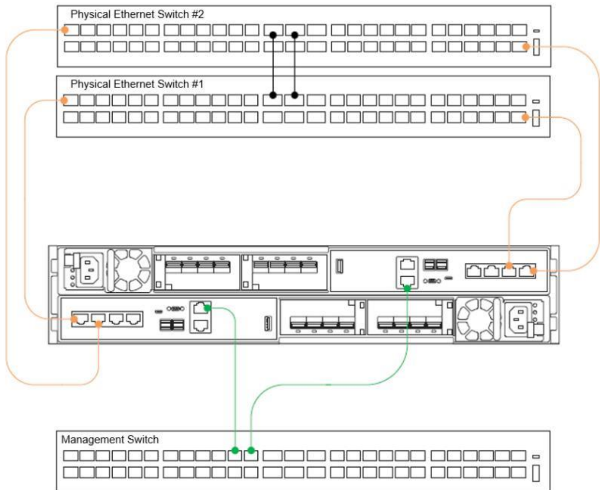
Figure 16 PowerStore T model appliance minimum cabling
